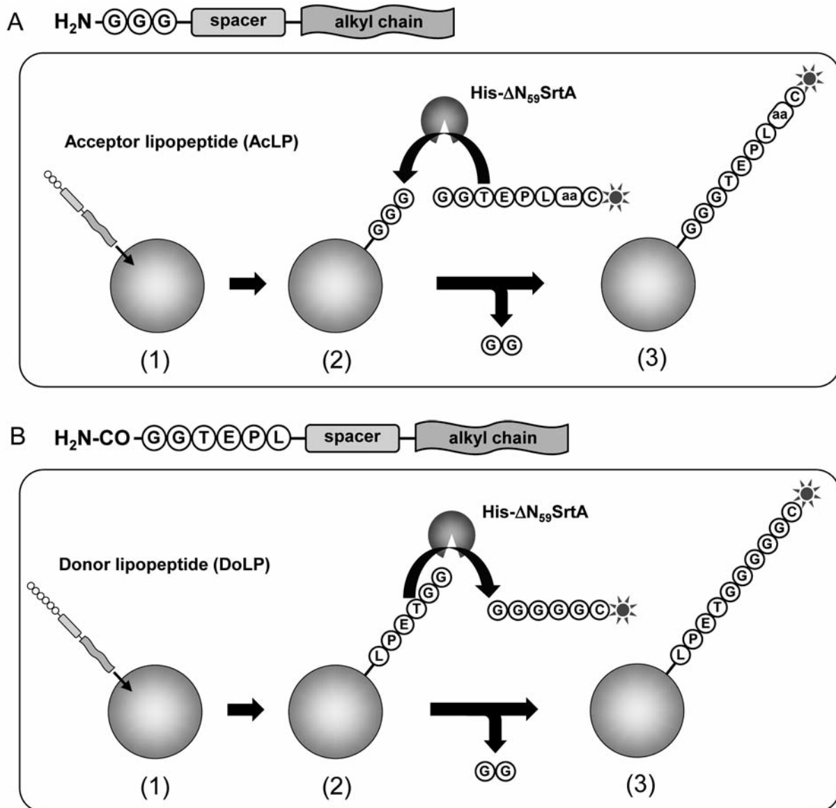
Figure 1. Schematic illustration of lipopeptide structure and strategy for evaluating His- \Delta\text{N}_{59} SrtA-mediated transpeptidation on lipopeptide-inserted DPPC-Chol-lipo. A: Acceptor lipopeptide (AcLP). The synthesized AcLP is composed of the acceptor oligoglycine and hexadecanoic acid with or without conjugated spacer (polyethylene glycol). Each AcLP was incubated with DPPC-Chol-lipo (step 1). Subsequently, the transpeptidase reaction mediated by His- \Delta\text{N}_{59} SrtA using a fluorescently labeled peptide (including the SrtA recognition sequence LPETG where some amino acids are described as “aa”) as donor substrate was conducted (step 2). Finally, the reaction product was evaluated by measuring the fluorescence intensity of resulting liposomes (step 3). In the present study, three AcLPs with different spacer structures were investigated. B: Donor lipopeptide (DoLP). The synthesized DoLP is composed of the donor sequence of SrtA (LPETG) and hexadecanoic acid with or without conjugated spacer (polyethylene glycol). Each DoLP was incubated with DPPC-Chol-lipo (step 1). Subsequently, His- \Delta\text{N}_{59} SrtA-mediated transpeptidation of the fluorescently labeled acceptor oligoglycine peptide was conducted (step 2). The reaction product was evaluated as described in A (step 3). In the present study, two DoLPs with different spacer structures were investigated.
