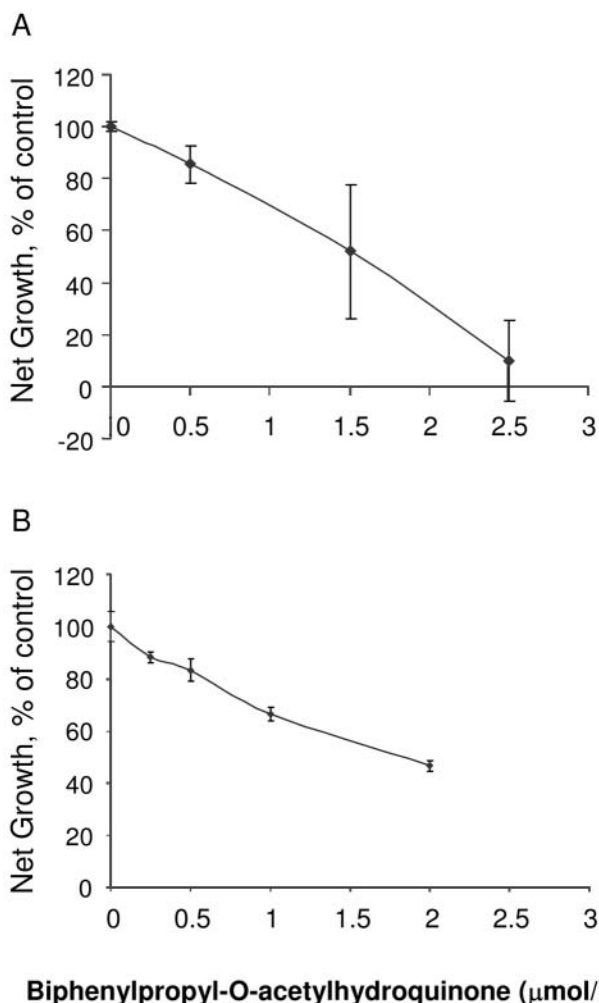
Figure 2. Representative growth curves of B16 melanoma cells showing the concentration-dependent suppression of B16 cell proliferation by biphenylpropyl-O-acetylhydroquinone. Cell proliferation was measured by CellTiter 96® Aqueous One Solution (A) and Guava® ViaCount® assay (B) after 48-h incubation. Values are mean \pm SD, n=3 .
